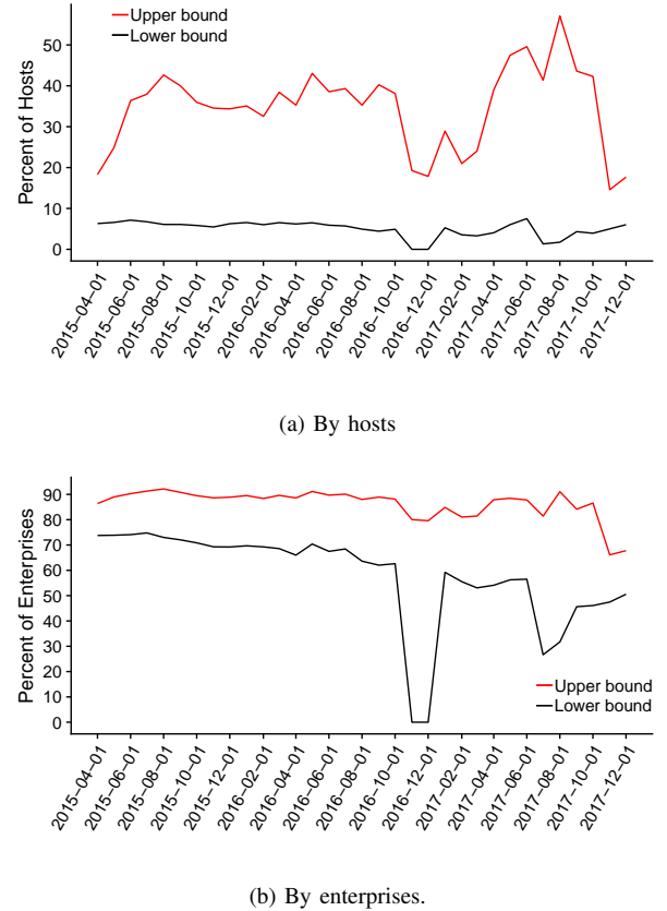
Fig. 2: Monthly malware and PUP prevalence measured by number of hosts and enterprises with at least one malicious encounter.
