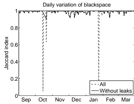
Fig. 4: Day-to-day variation of the blackspace prefixes.
